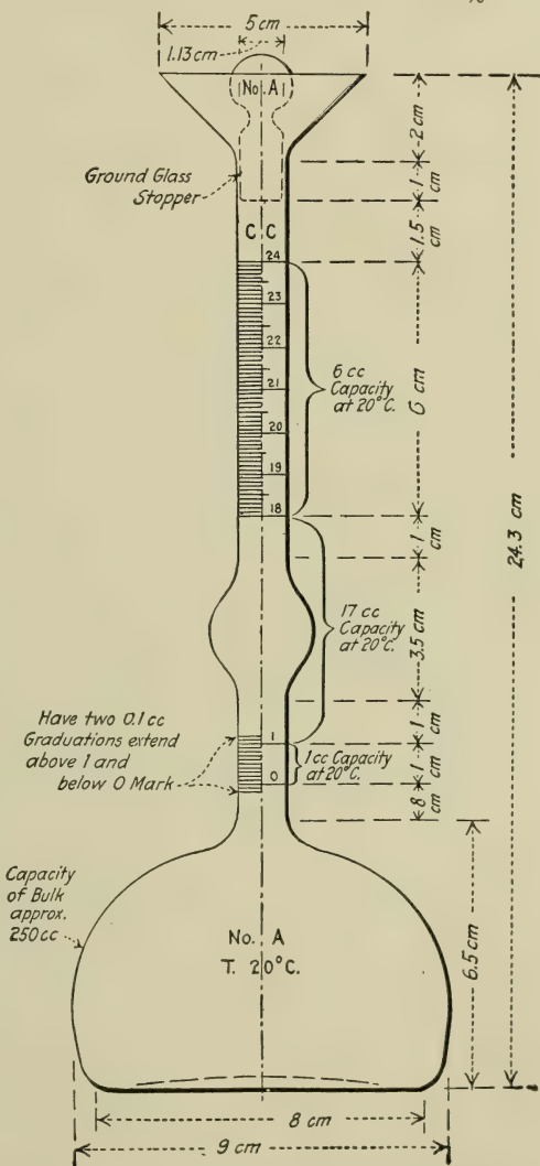
From A. S. T. M. Standards. FIG. 191.—Bureau of Standards' Modification of Le Chatelier's Specific Gravity Flask.
